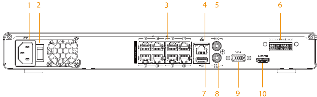
Rear panel (8-PoE port)
